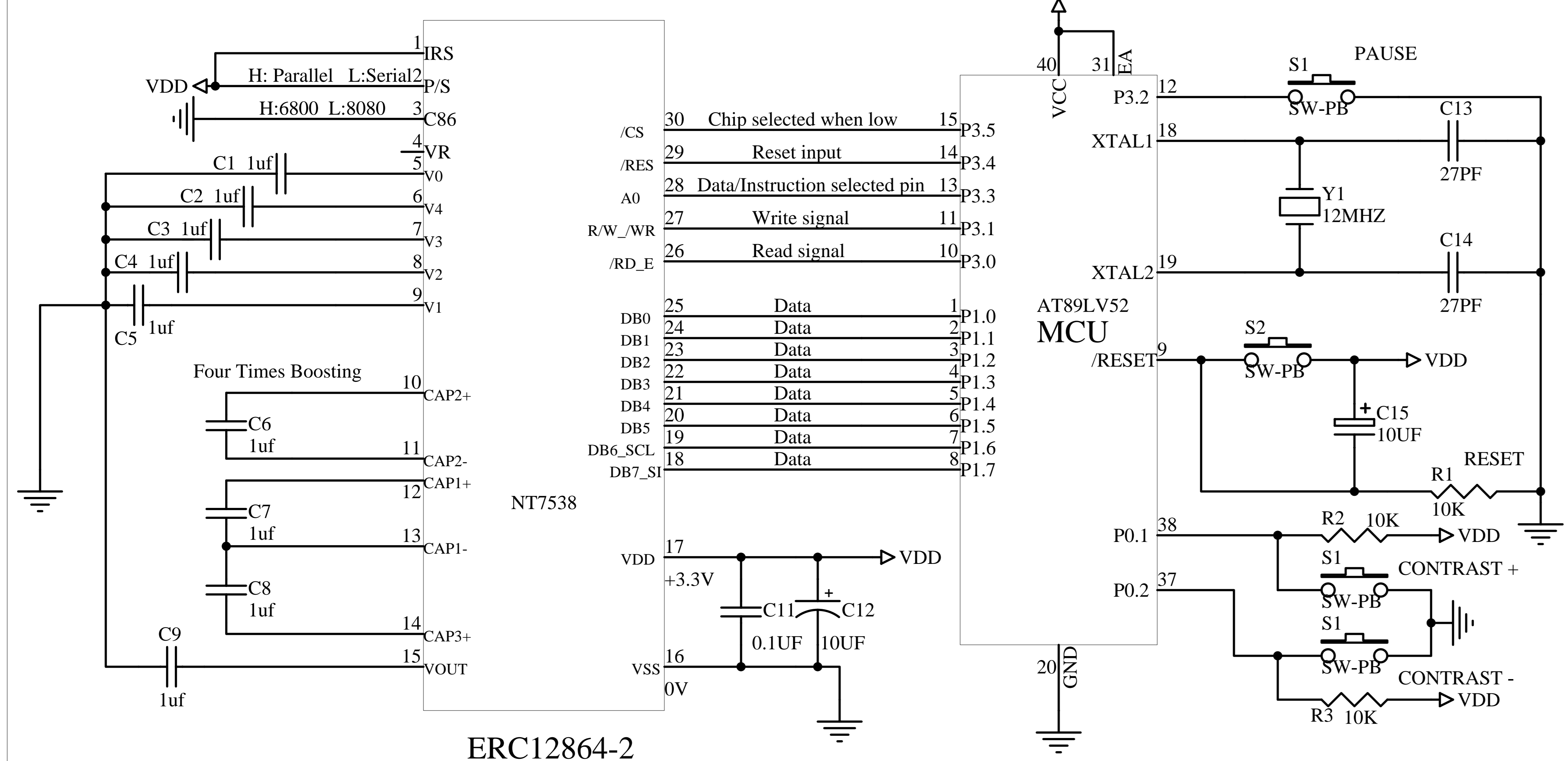
The Parallel (8080 Series MCU Reference Example)
