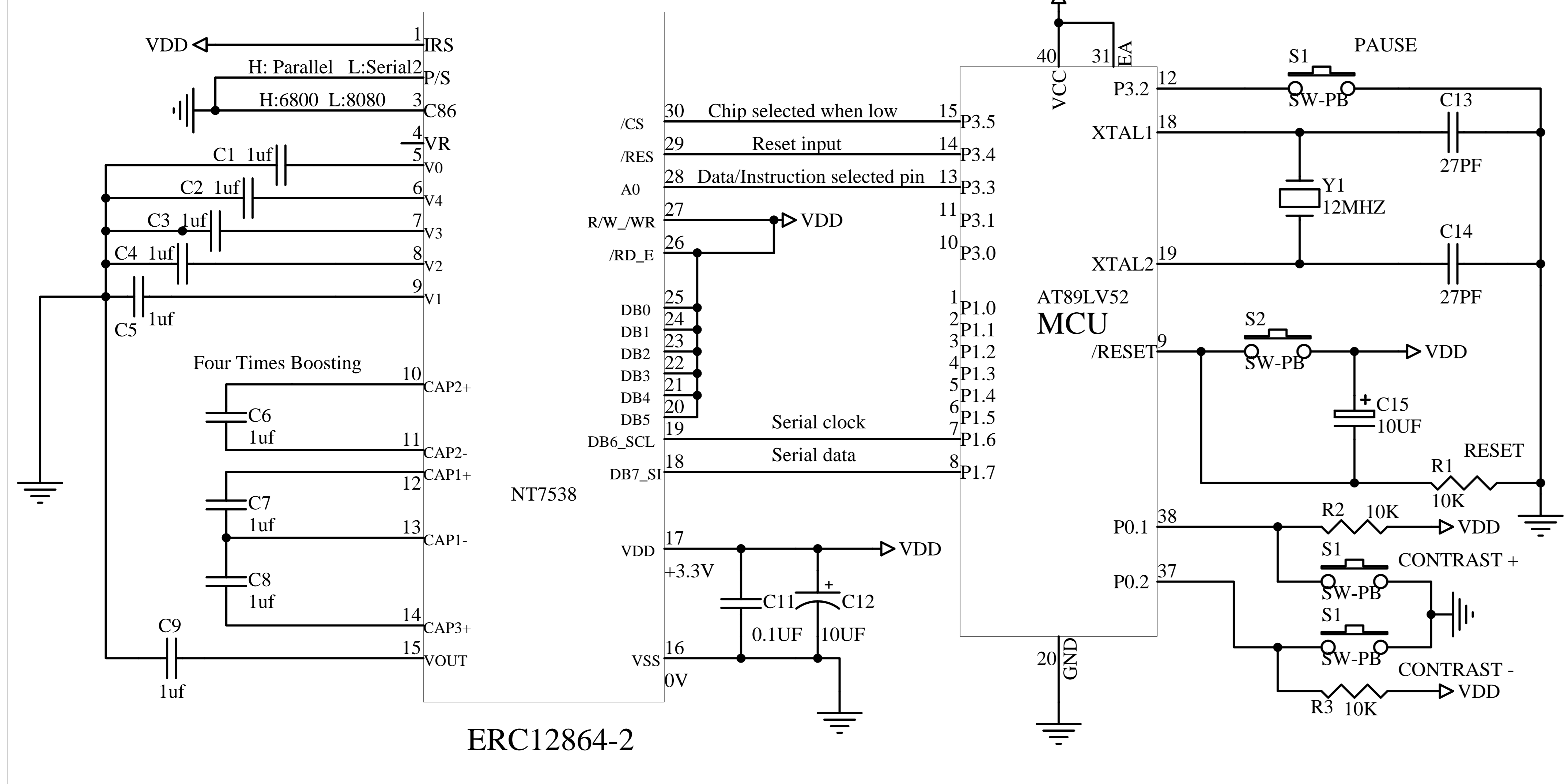
The Serial (SPI) Reference Example
