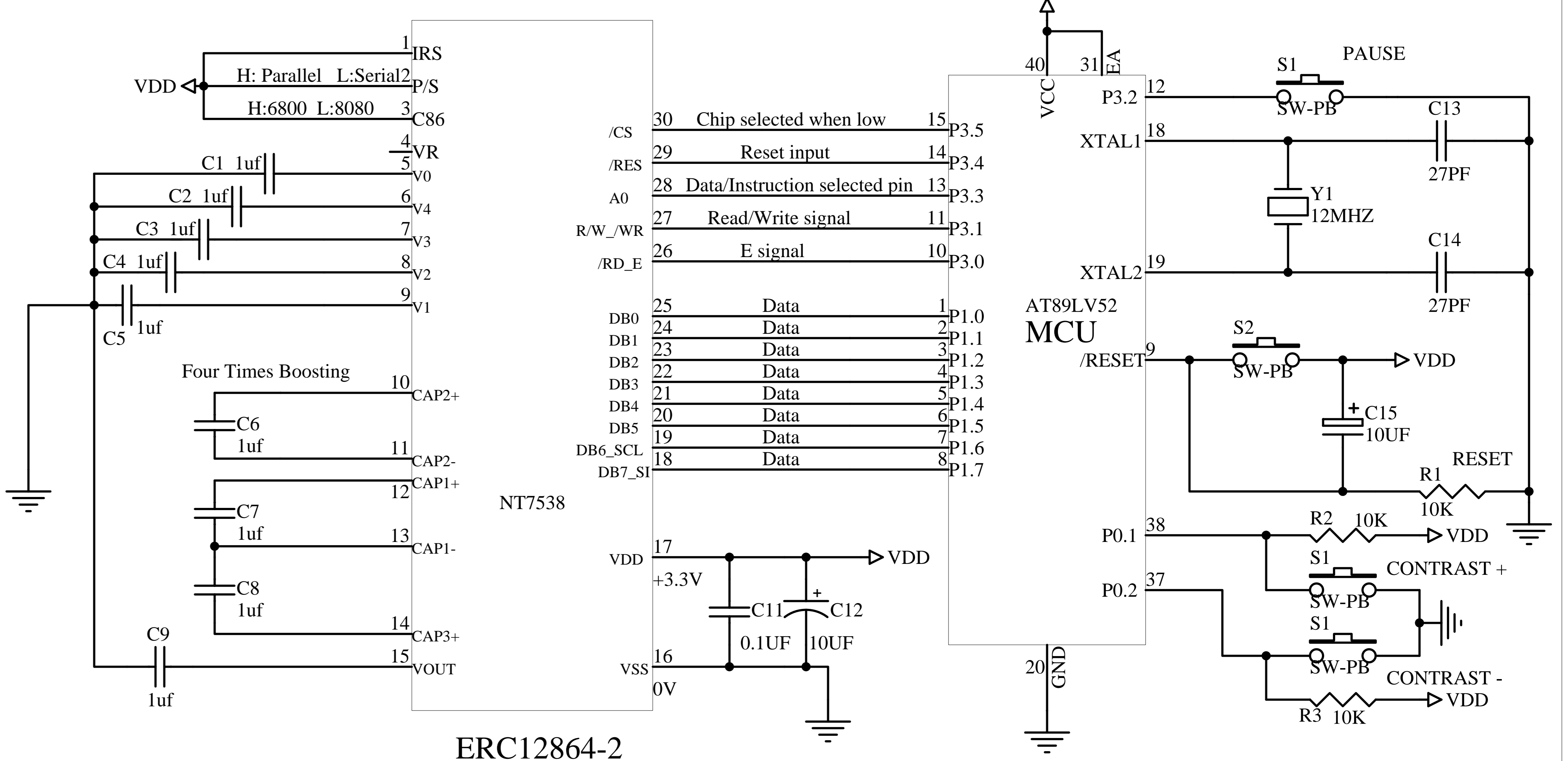
The Parallel (6800 Series MCU) Reference Example
