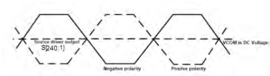
Relationship between Source Output and VCOM
