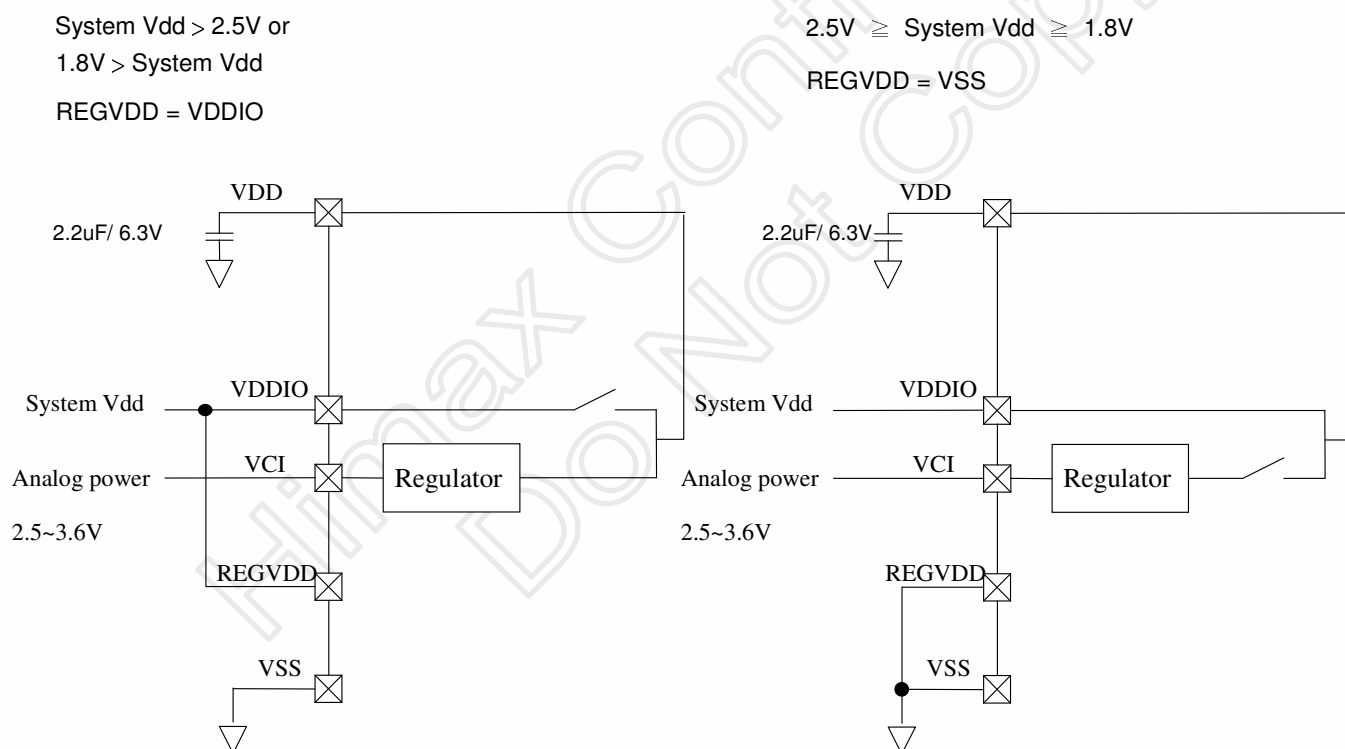
Figure 16.1 Booster capacitors
