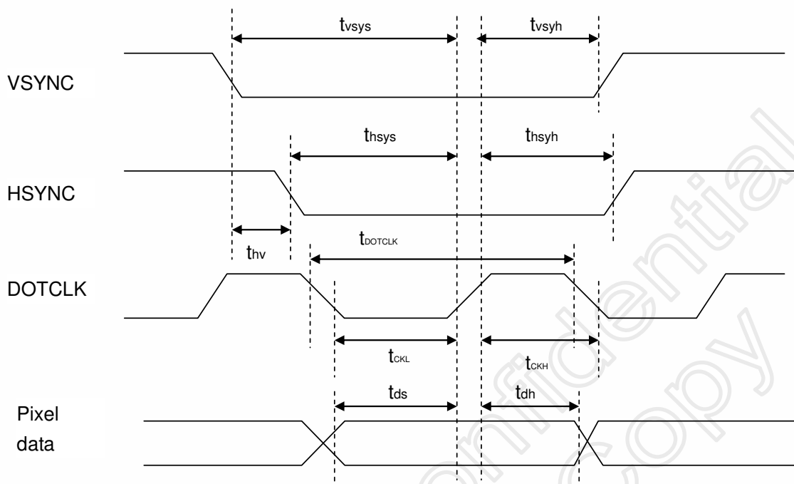
Figure 14. 1 Pixel timing
