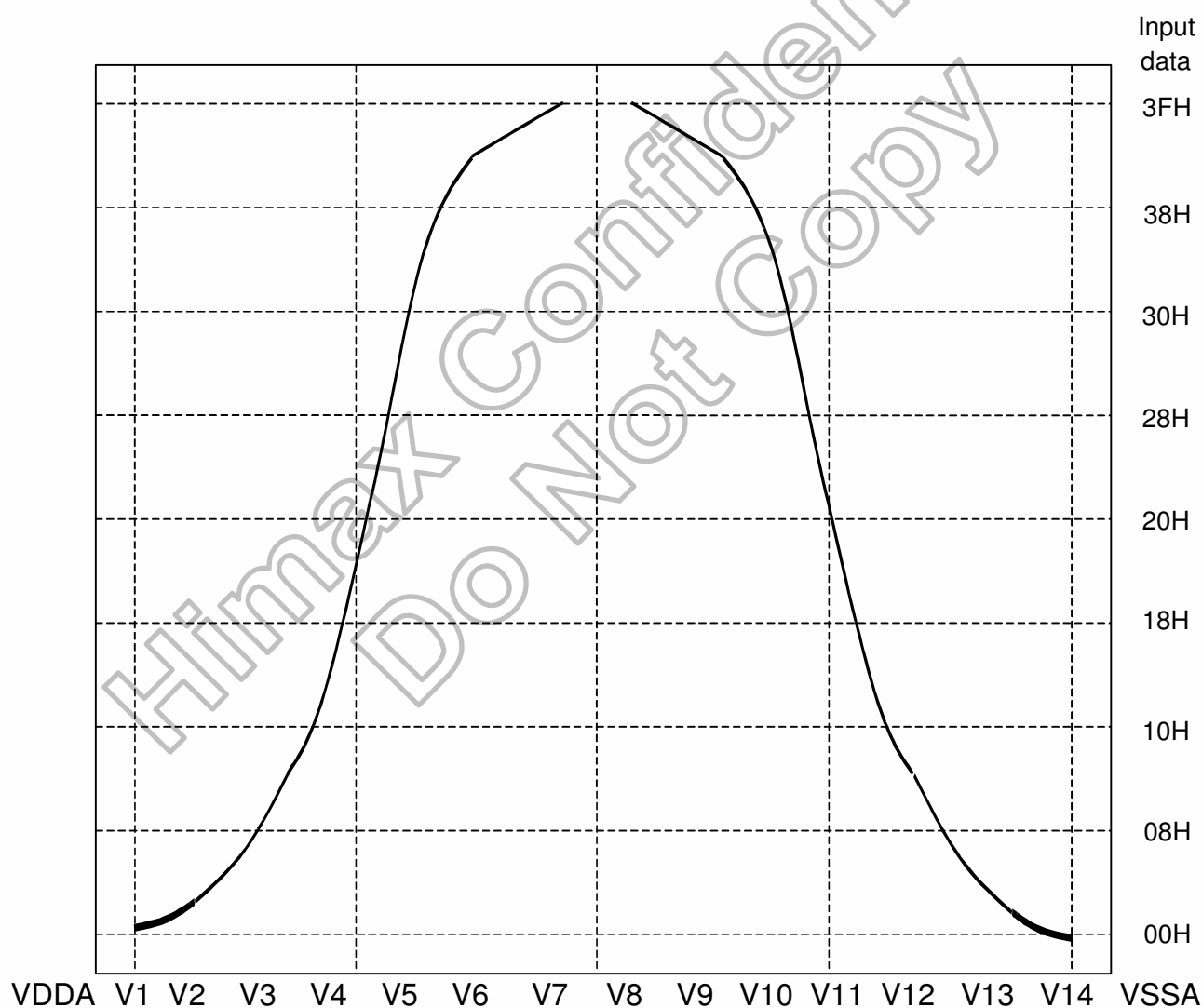
Figure 6. 1: Gamma Correction Characteristic Curve
