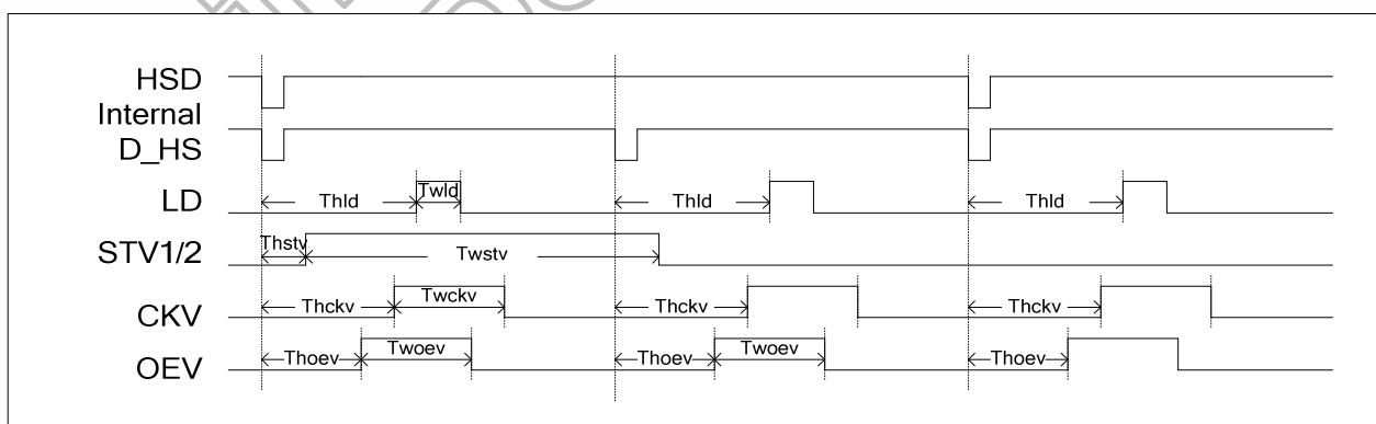
Figure 12. 9: Gate Output Timing Diagram (Dual Gate)
