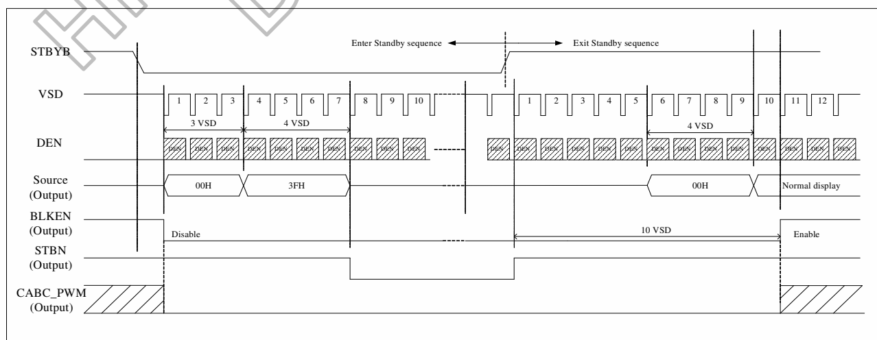
Figure 9. 2: Enter and Exit Standby Mode Sequence
