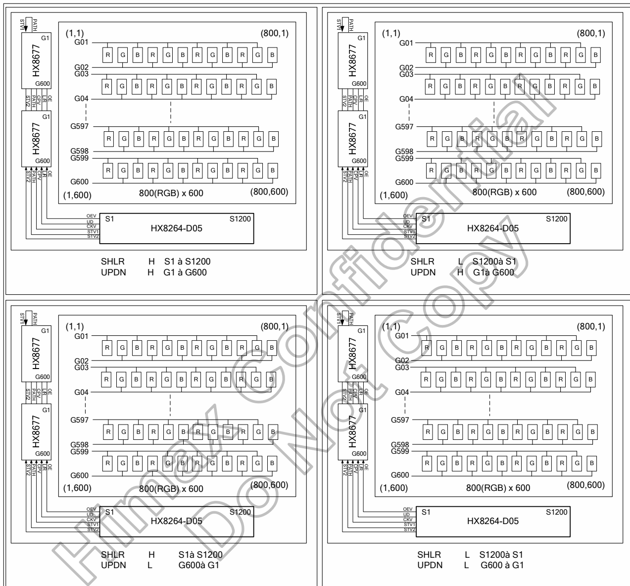
Figure 3. 8: HX8264-D05 Dual Gate 800(RGB) x 600 Application Block Diagram-1
