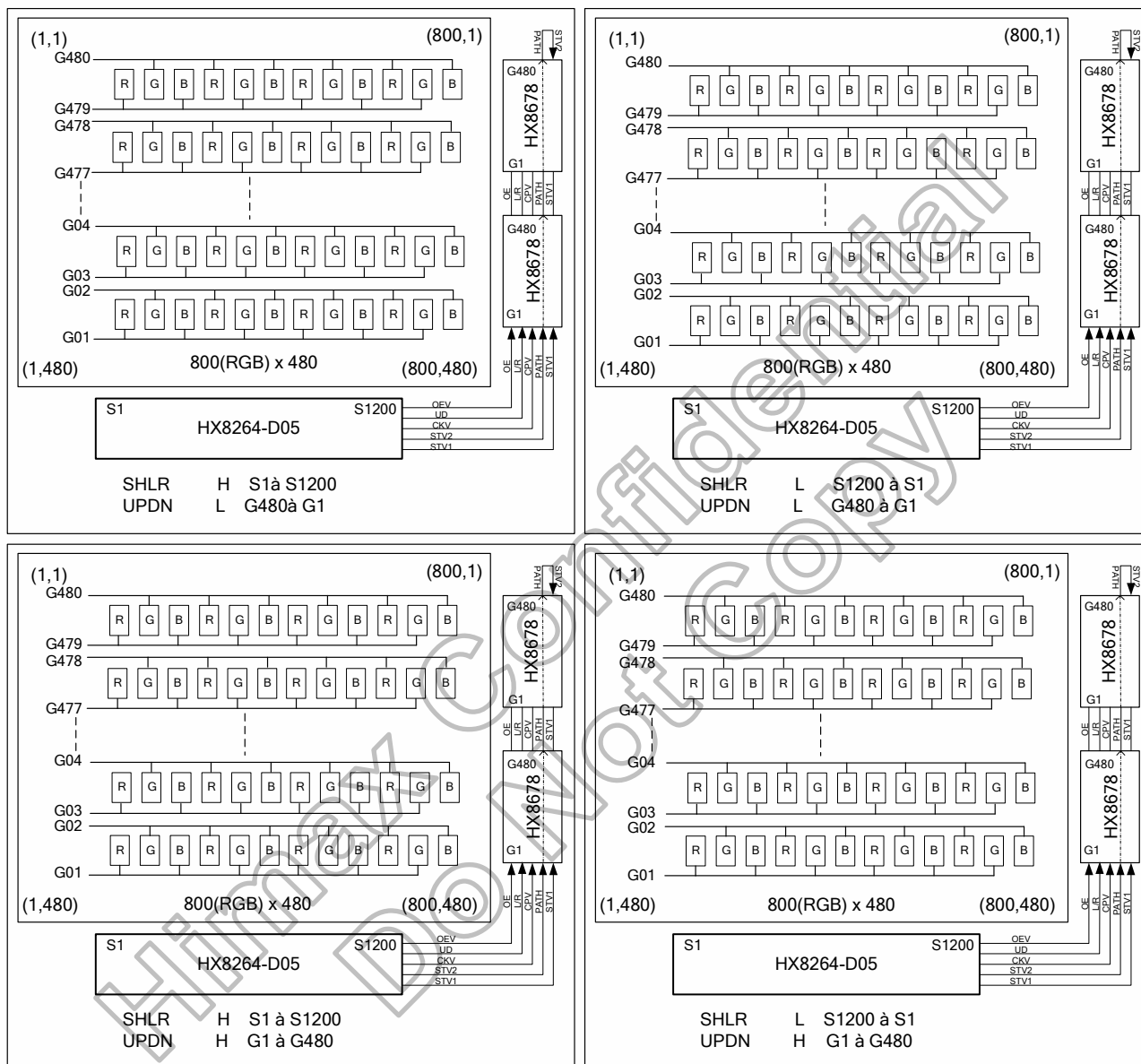
Figure 3. 7: HX8264-D05 Dual Gate 800(RGB) x 480 Application Block Diagram-2
