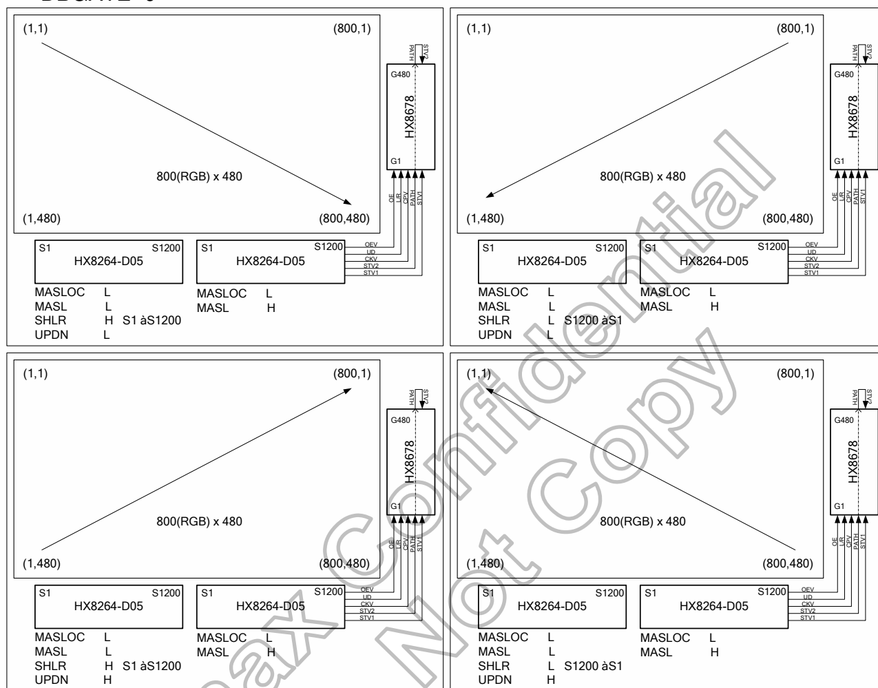
Figure 3.3 HX8264-D05: Two Chip Cascade 800(RGB) x 480 Application Block Diagram-2
