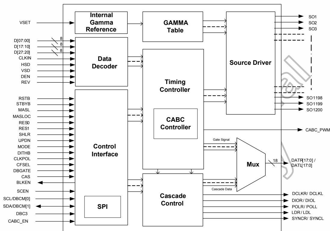
Figure 3. 1: HX8264-D05 Function Block Diagram
