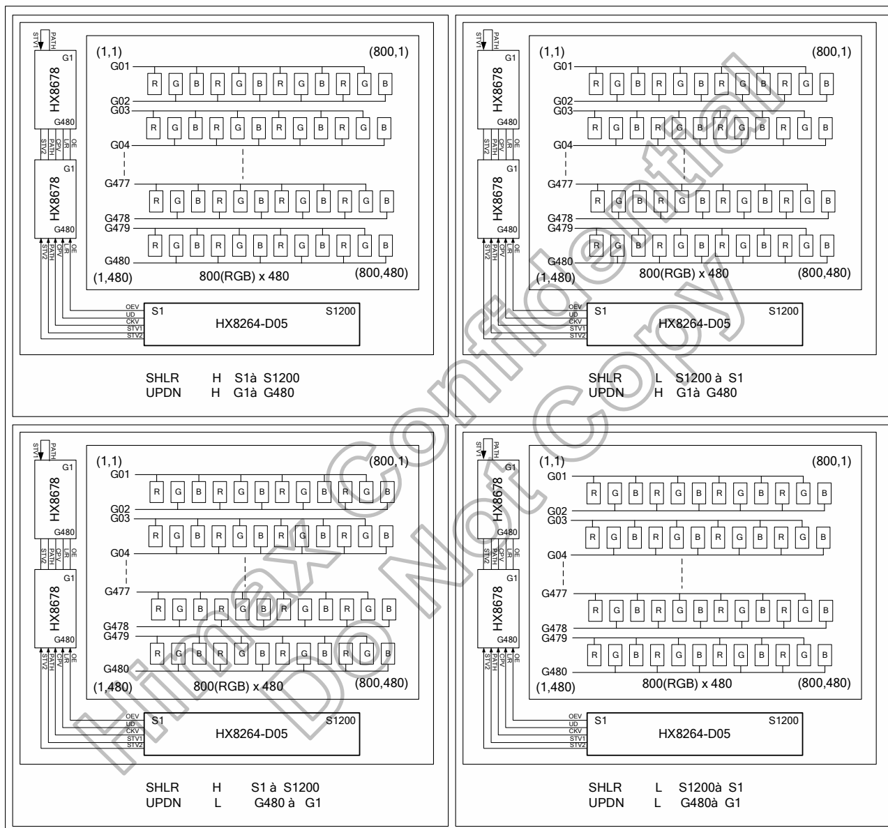
Figure 3. 6: HX8264-D05 Dual Gate 800(RGB) x 480 Application Block Diagram-1
