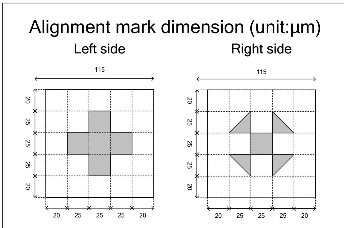
Figure 14. 2: Alignment Mark
