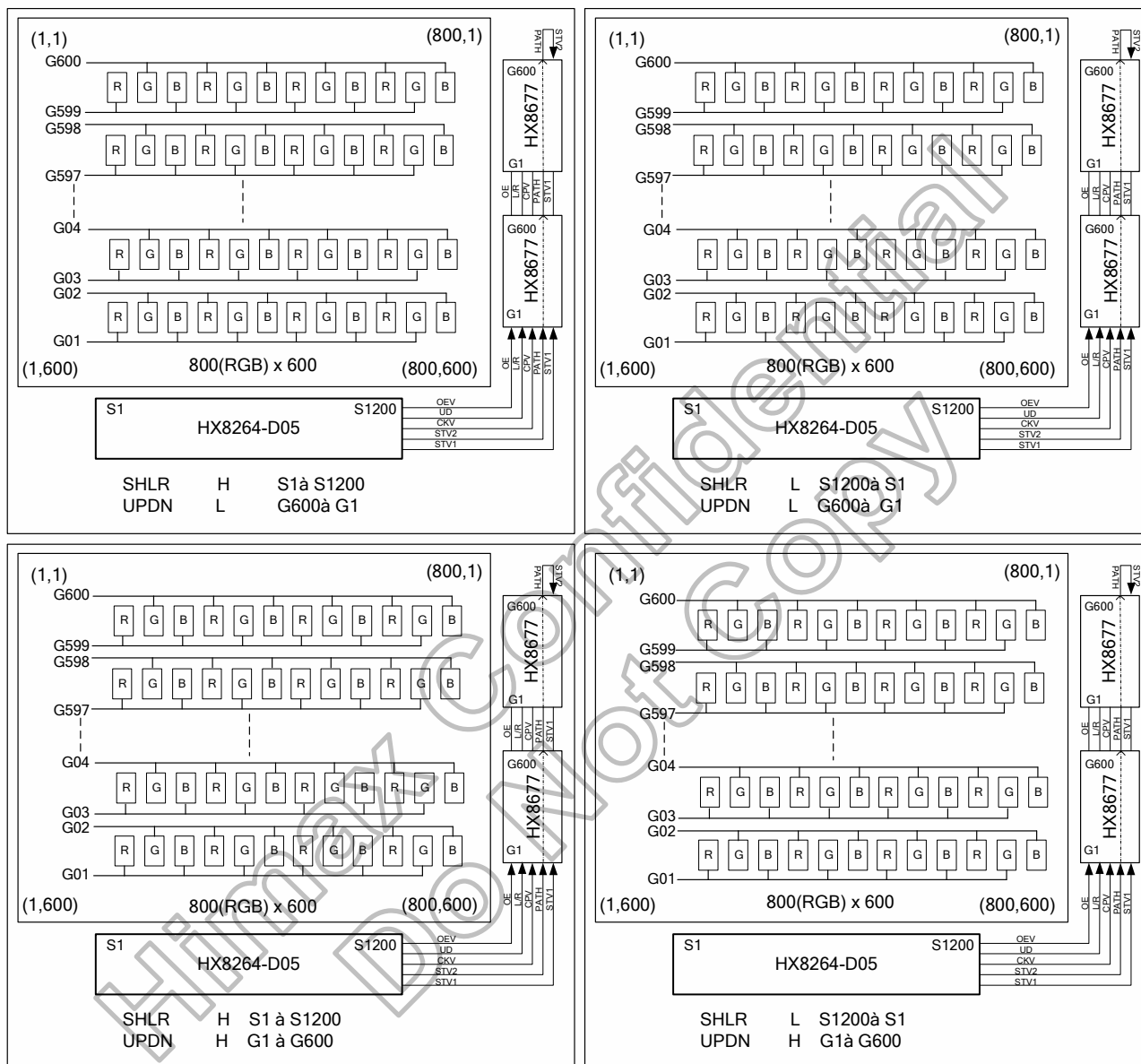
Figure 3. 9: HX8264-D05 Dual Gate 800(RGB) x 600 Application Block Diagram-2
