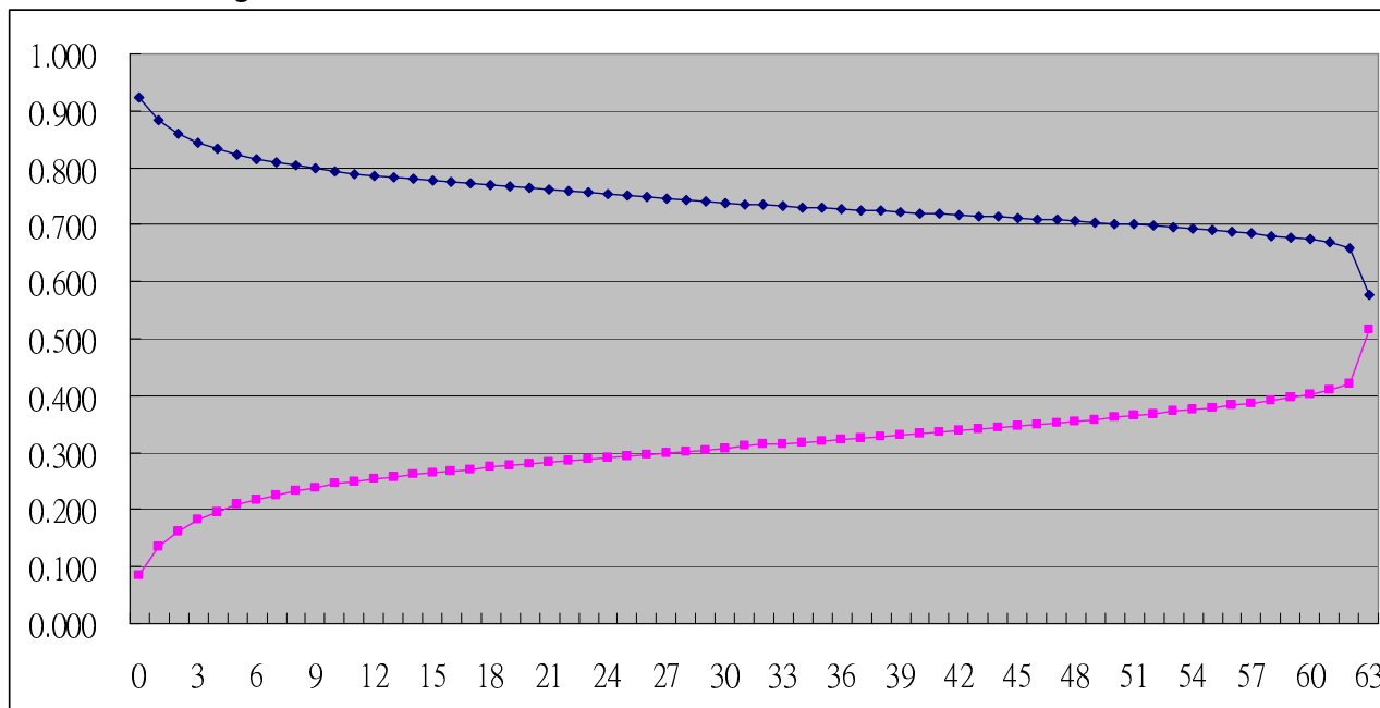
Figure 6.1: Gamma curve
