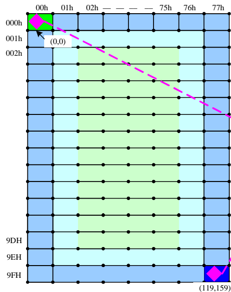
GRAM size(120x160x18-bits)
