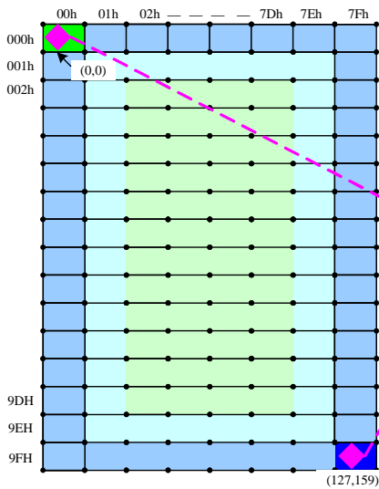
GRAM size(128x160x18-bits)
