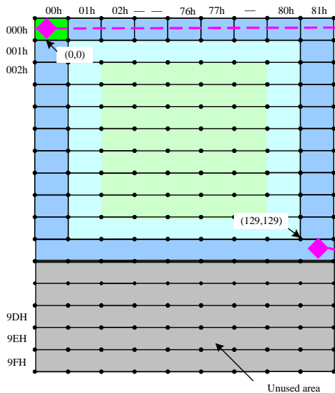
GRAM size(130x130x18-bits)
