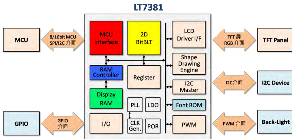
Figure A-1: Internal Block Diagram
