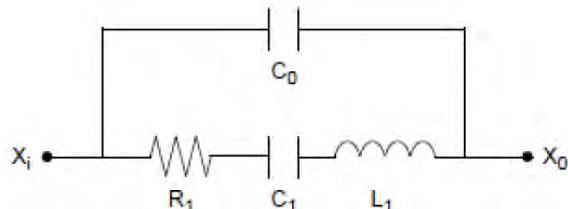
Figure A-4: Equivalent Circuit
