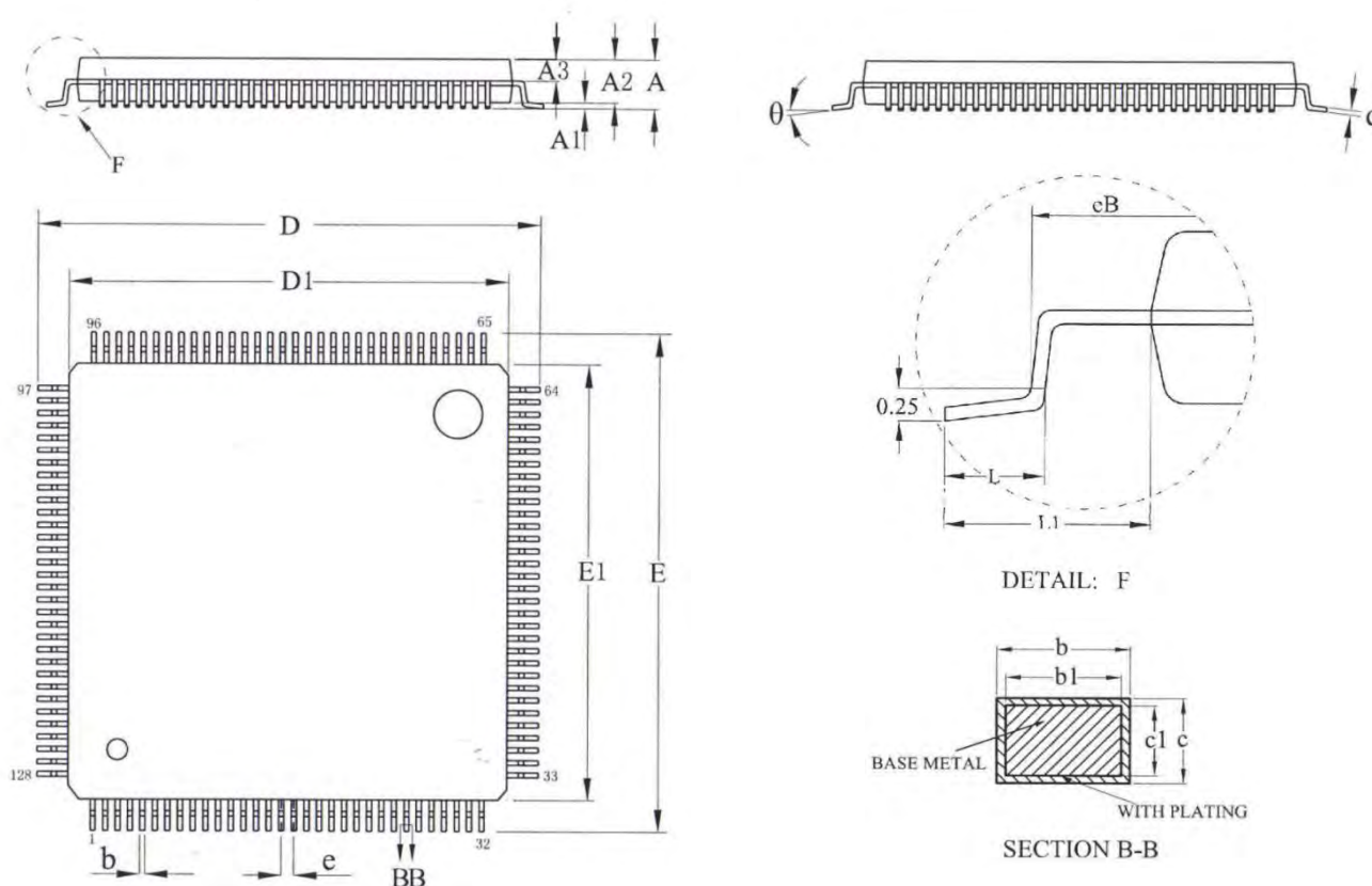
Figure B-1: 128Pin LQFP Outline
