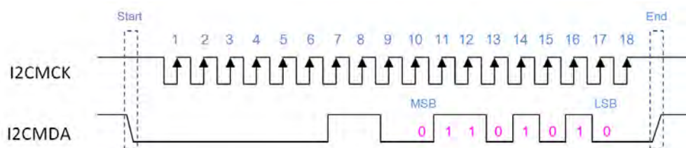
Figure 10-6: Read Data "6A" from Slave (Address=0x01)
