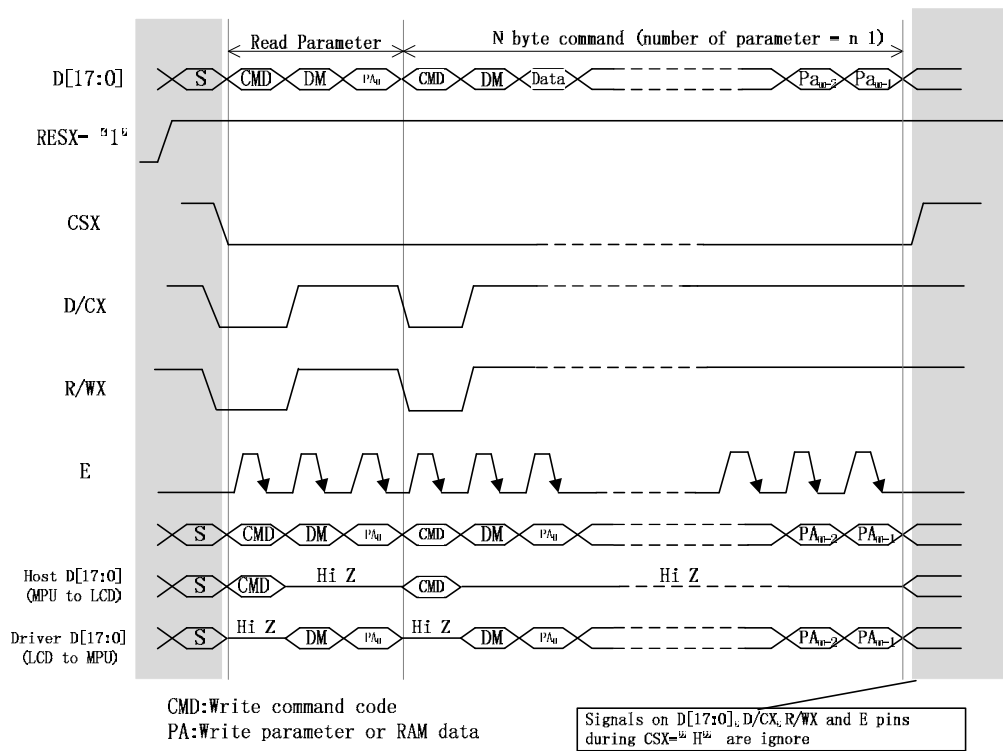
Figure 4-4-2 6800 Read Sequence
