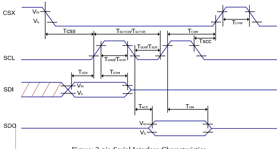
Figure: 3-pin Serial Interface Characteristics
