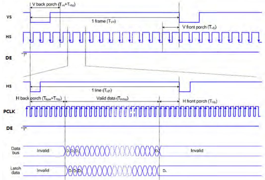
Timing chart of RGB interface SYNC mode
