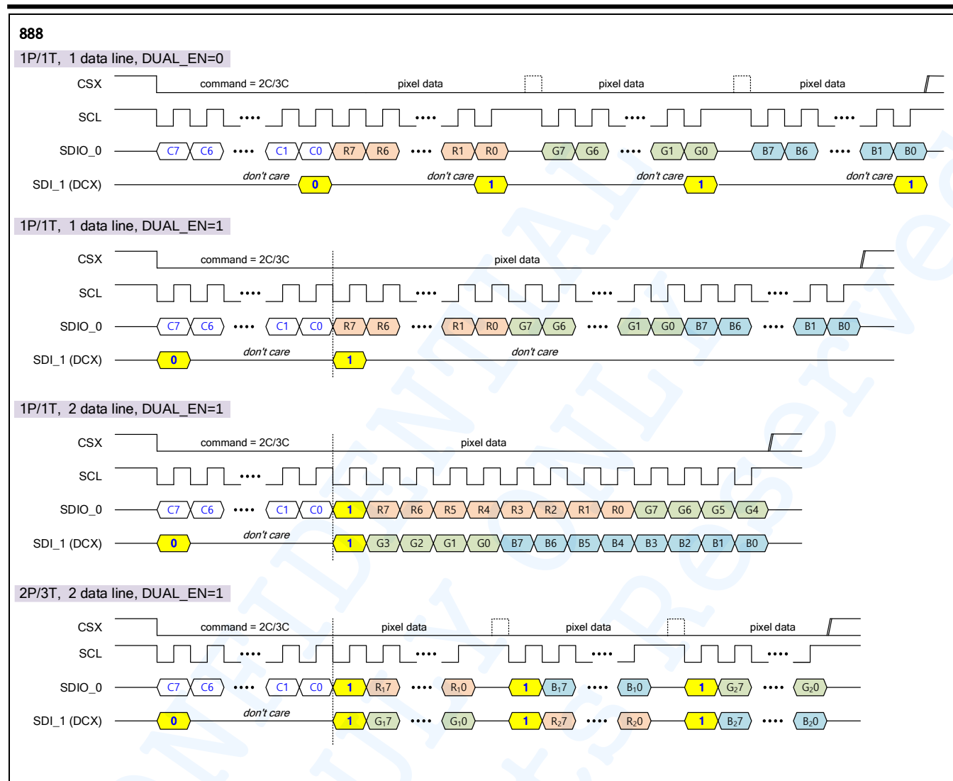
Figure 30 SPI 4-Wire 888 Pixel Format
