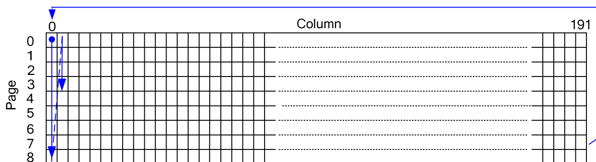
Fig 15. DDRAM Access Mapping (MX=0, AC[2:0]=3, PA[3:0]=0, CA[3:0]=0)
