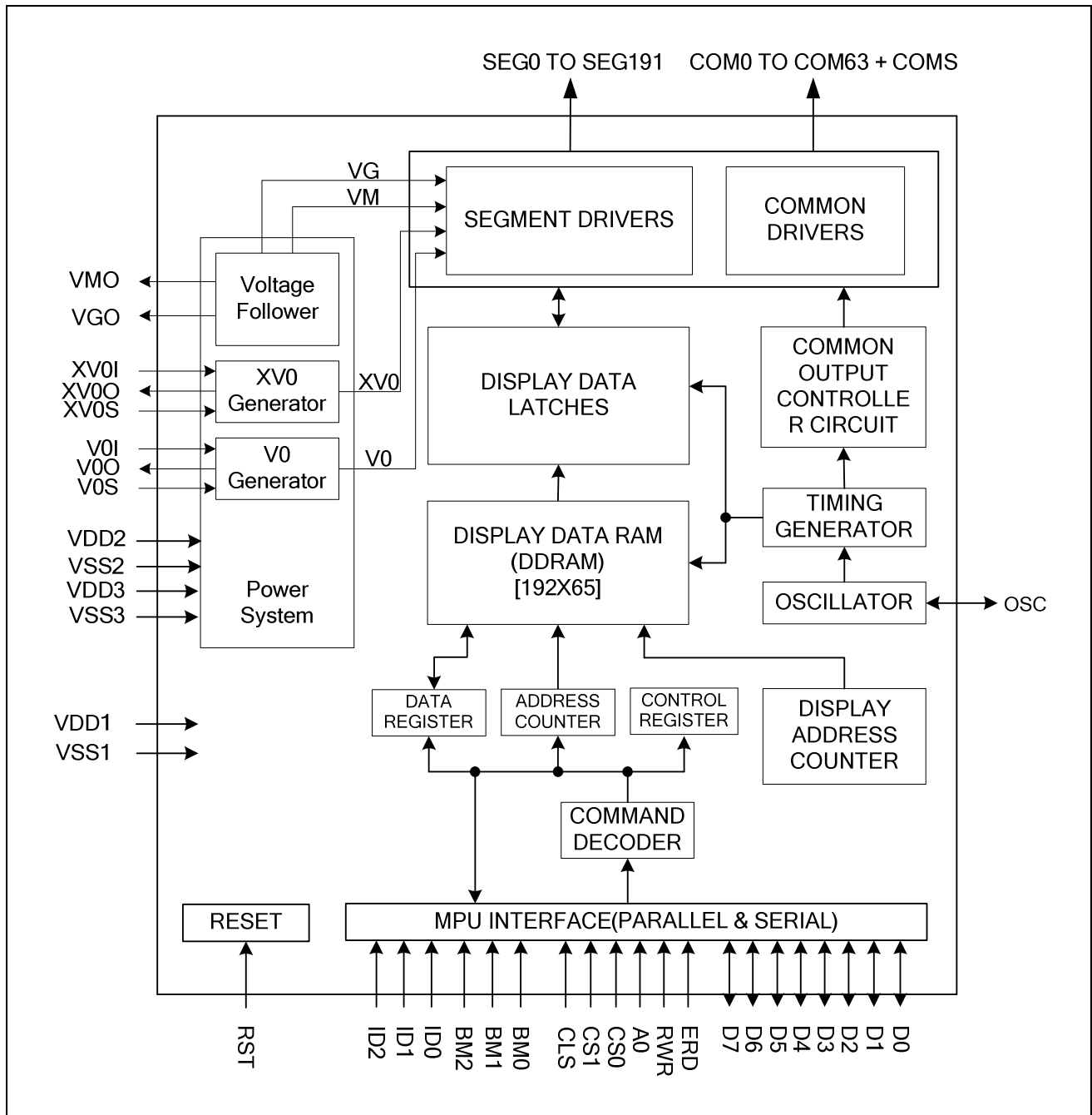
Fig 2. Block Diagram
