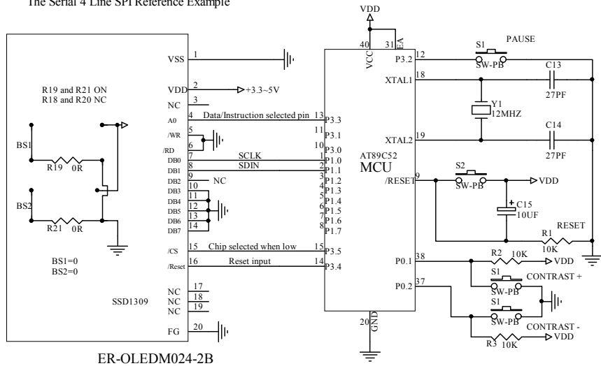
The Serial 4 Line SPI Reference Example
