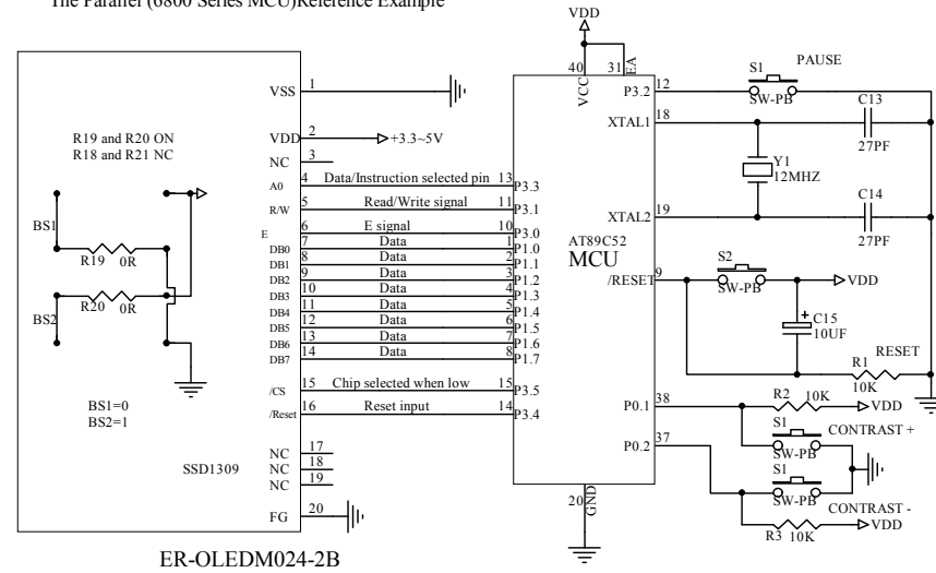
The Parallel (6800 Series MCU) Reference Example
