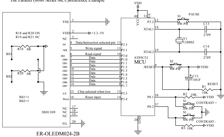
The Parallel (8080 Series MCU) Reference Example
