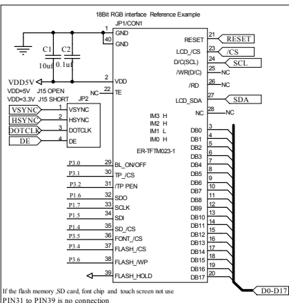
RGB Interfacing LCD Modules to the LCD Controller or Built-in LCD controller MCU
