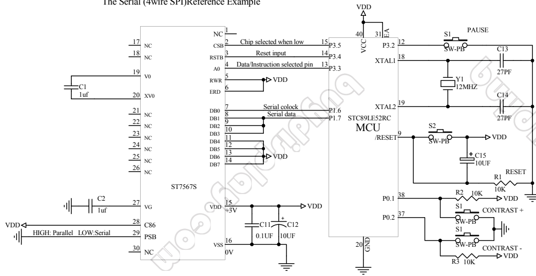
The Serial (4wire SPI)Reference Example
