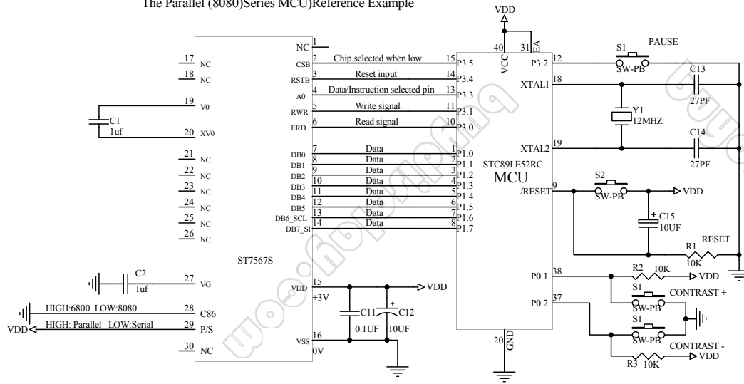
The Parallel (8080)Series MCU)Reference Example
