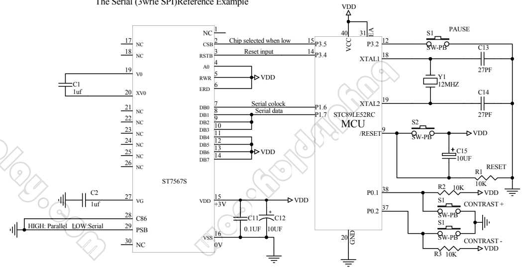
The Serial (3wire SPI)Reference Example
