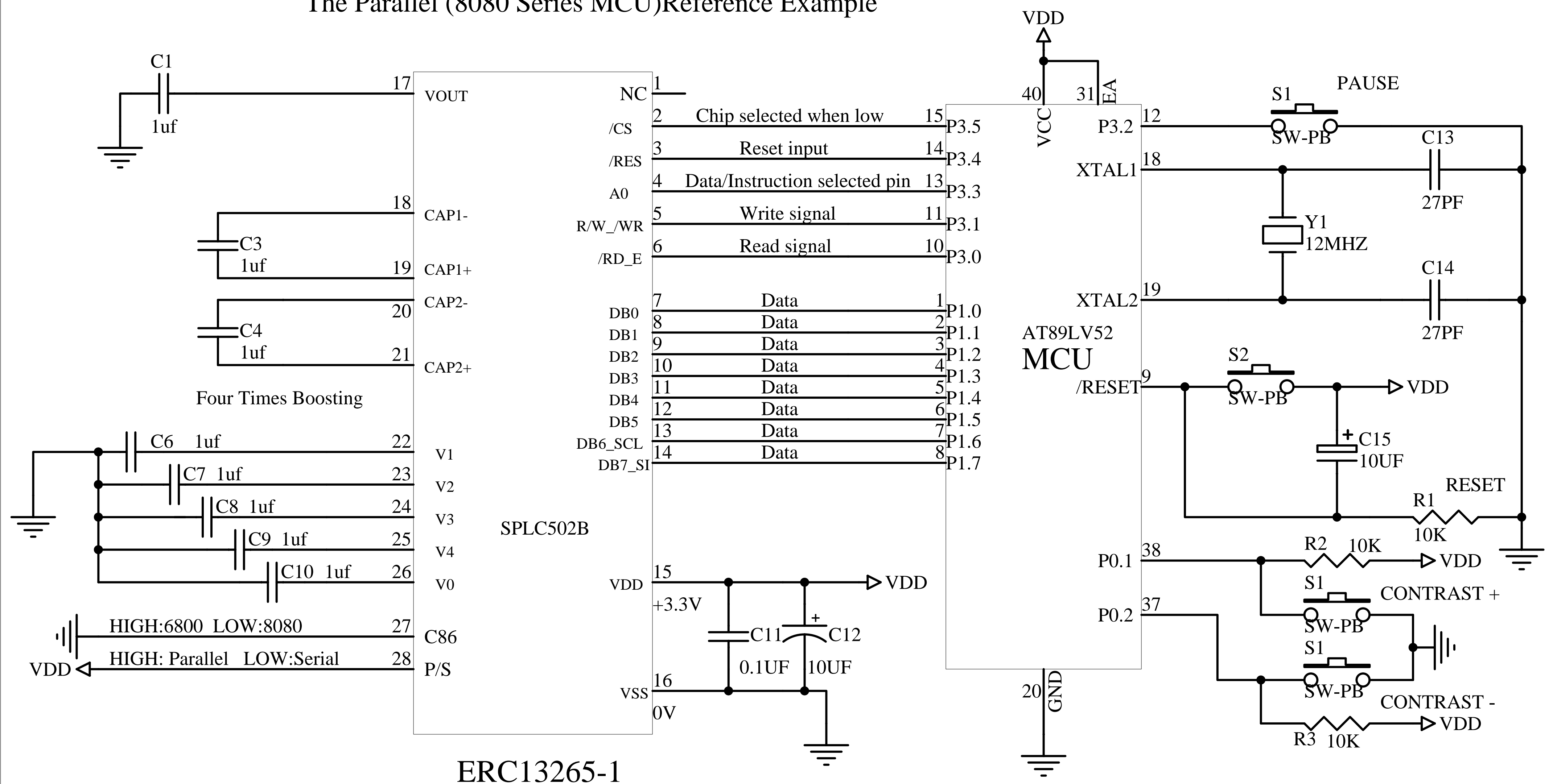
The Parallel (8080 Series MCU)Reference Example
