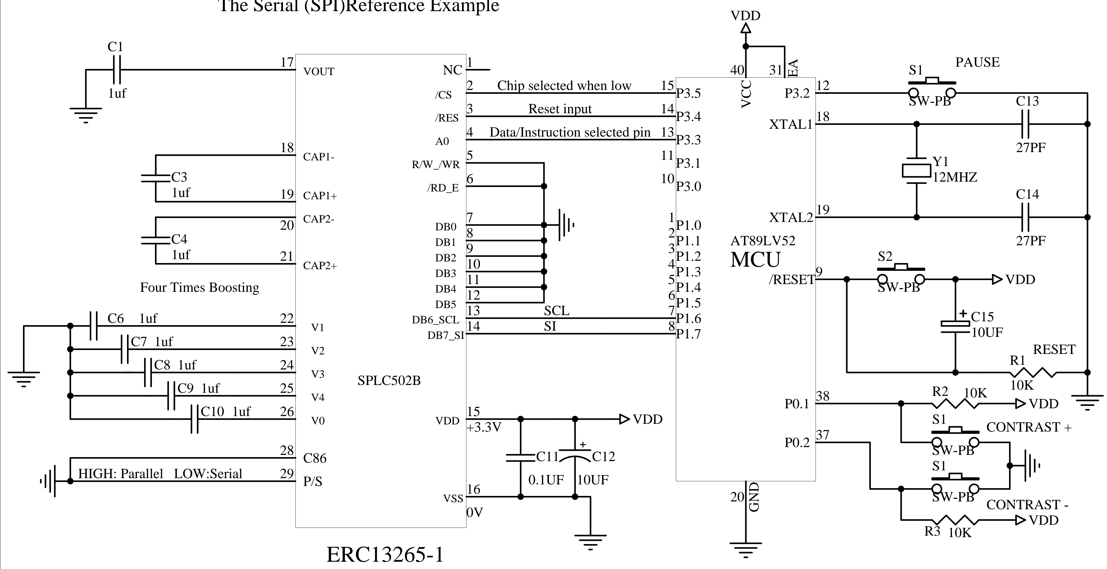
The Serial (SPI)Reference Example
