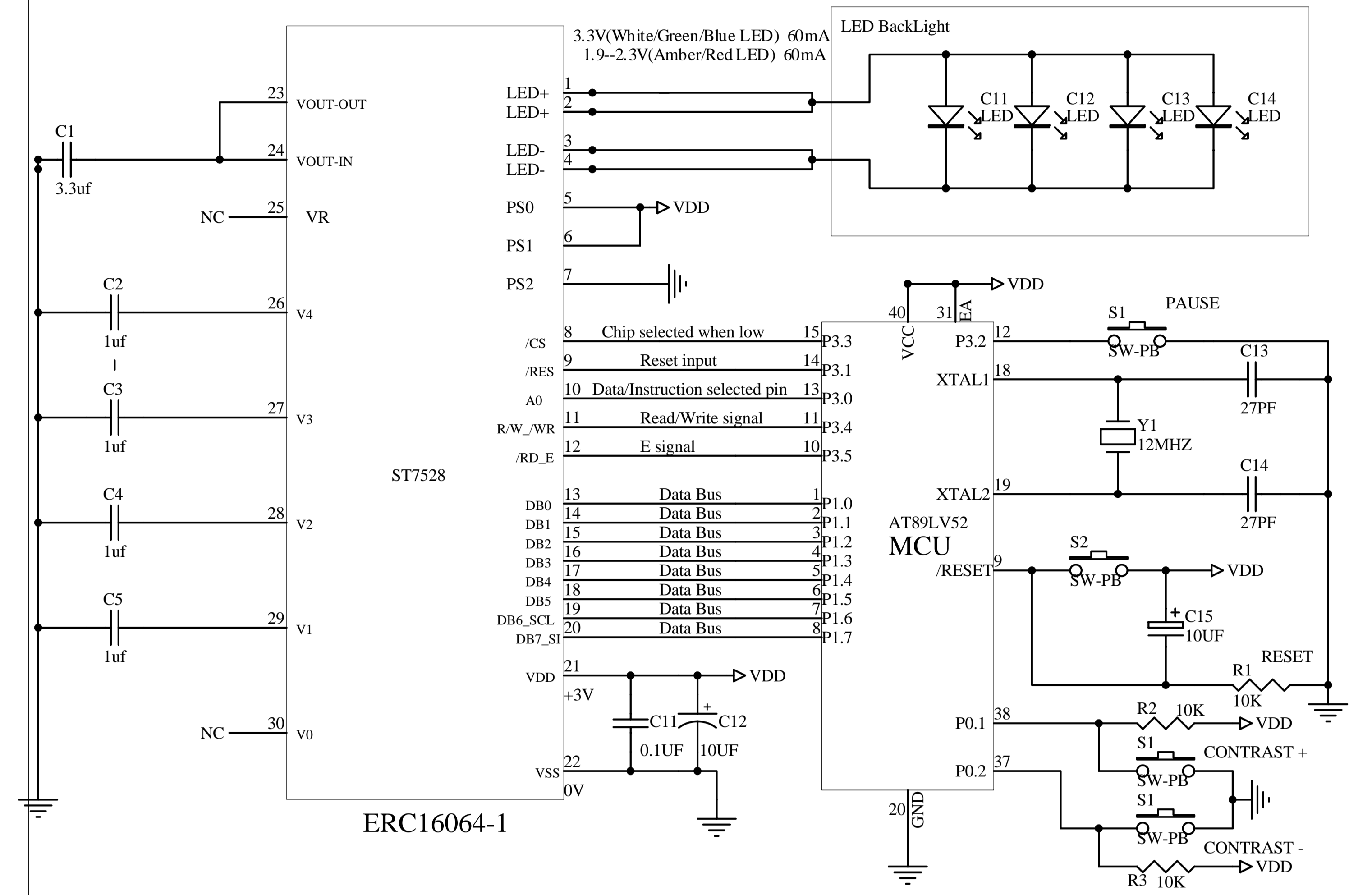
The Parallel 8Bit(6800 Series MCU)Reference Example
