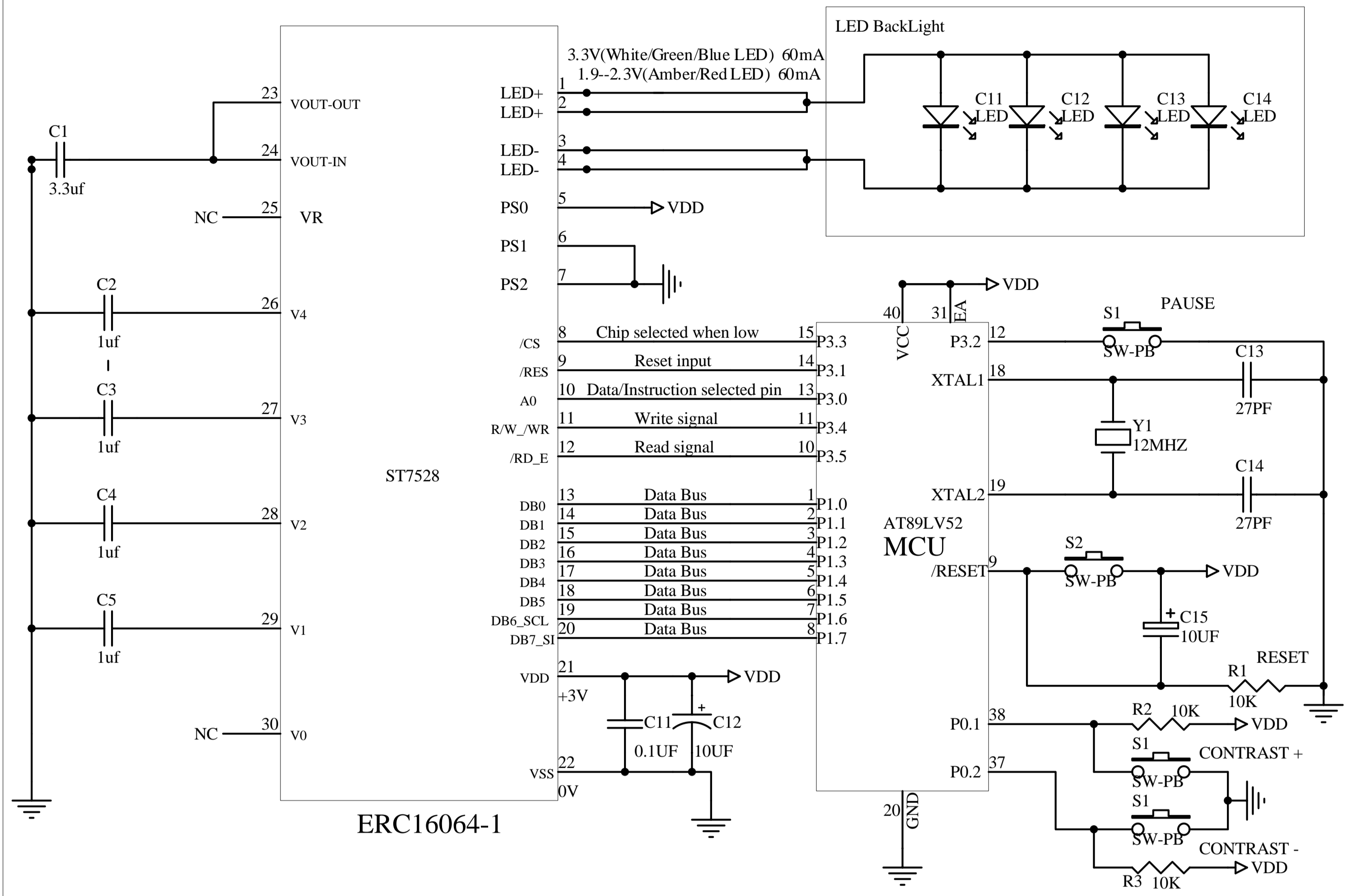
The Parallel 8Bit(8080 Series MCU)Reference Example
