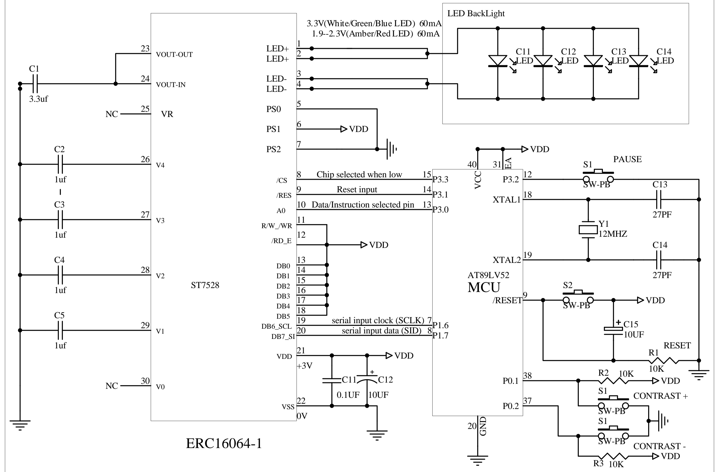
The Serial 4line SPI Reference Example
