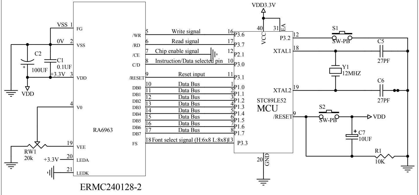
The 3.3V power supply, Parallel 8Bit(8080 Series MCU)Reference Example
