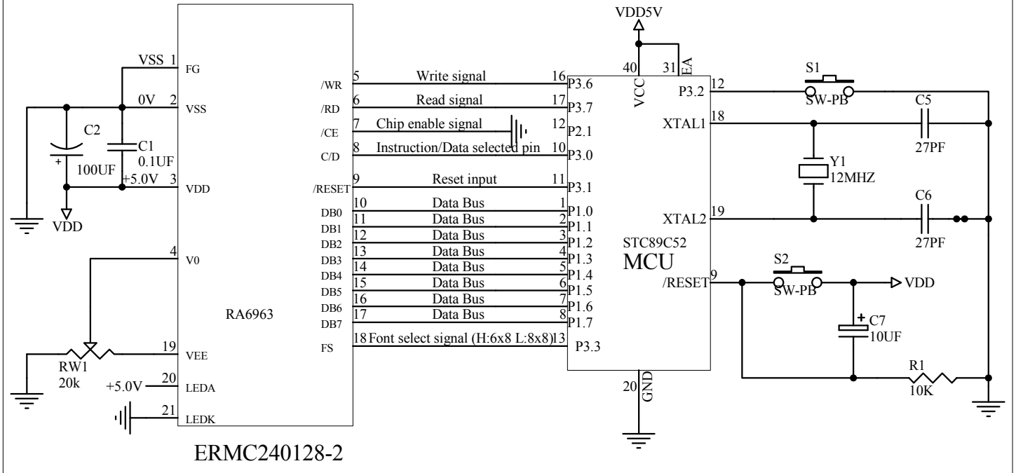
The 5V power supply, Parallel 8Bit(8080 Series MCU)Reference Example
