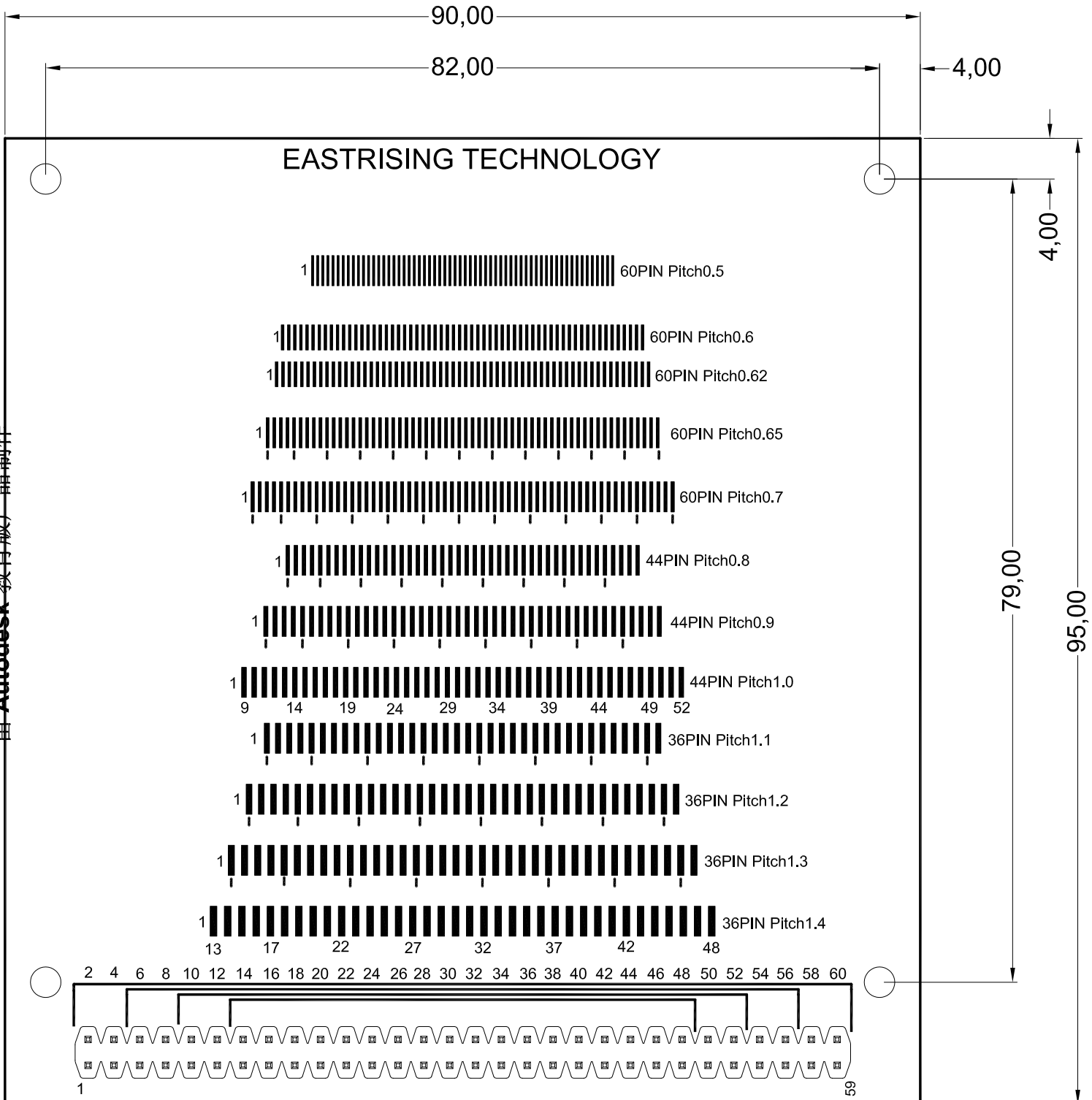
Adaptor Board ↑
