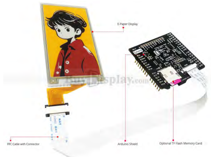
ER-EPD037-2RY-5070 ↓
