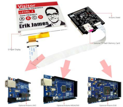
ER-EPD042A1-1R-5103 ↓
