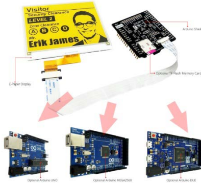
ER-EPD042-1Y-5103 ↓
