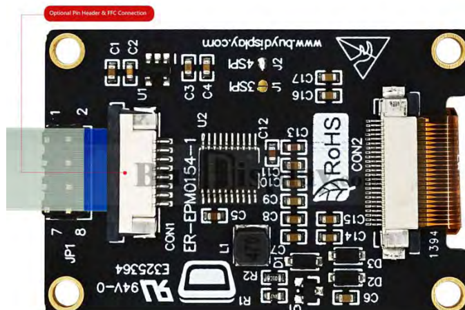
ER-EPM0154-1 Bottom_View ↓
