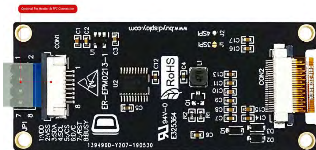
ER-EPM0213-1 Bottom_View ↓
