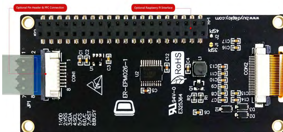
ER-EPM026-1 Bottom_View ↓
