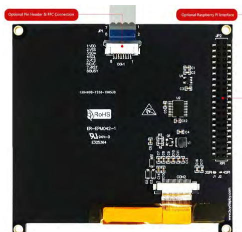
ER-EPM042A2-1 Bottom View ↓
