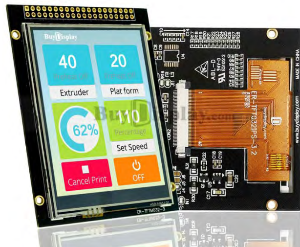
← ER-TFT032IPS-3.2-4334 with Capacitive Touch Panel
