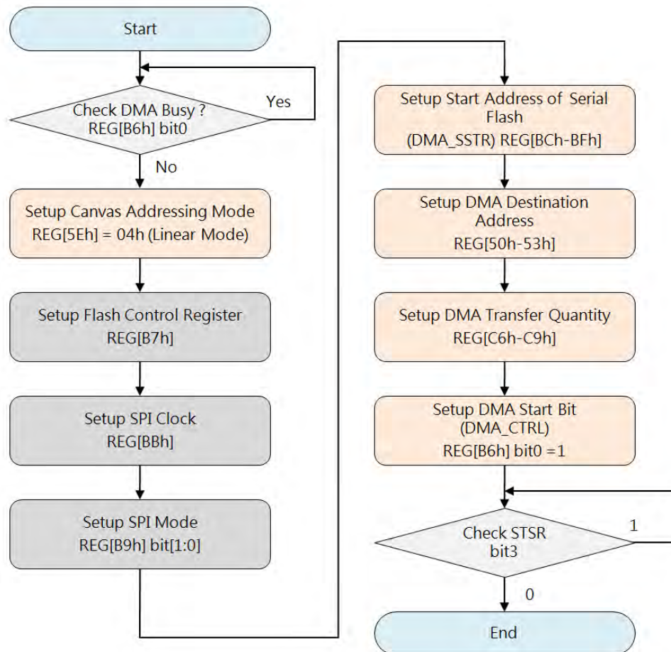
Figure 8-3: Flow Chart of CGRAM Initialization from Serial Flash
