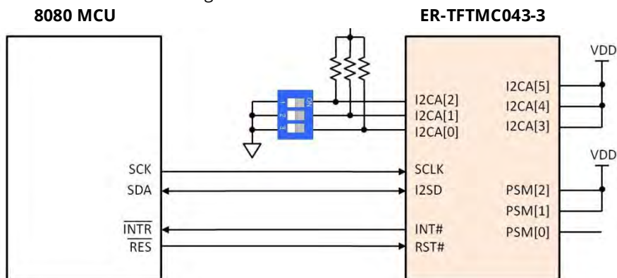
Figure 2-10: I2C Interface
