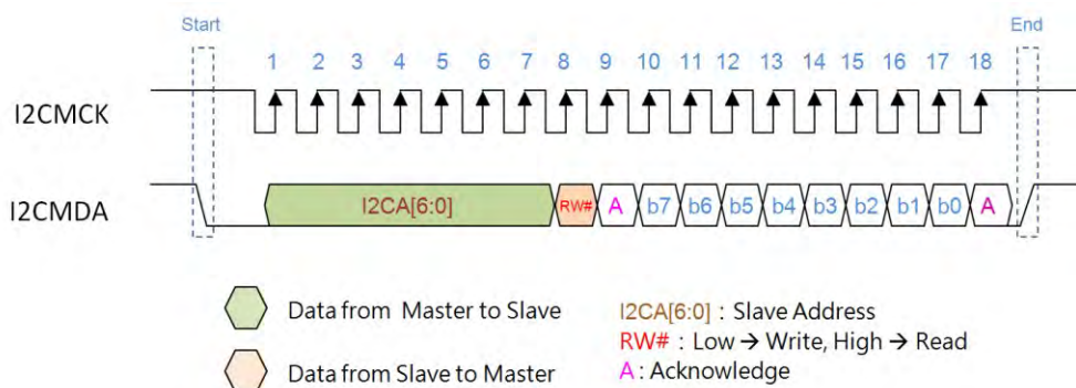
Figure 10-2: I2C Communication Protocol
