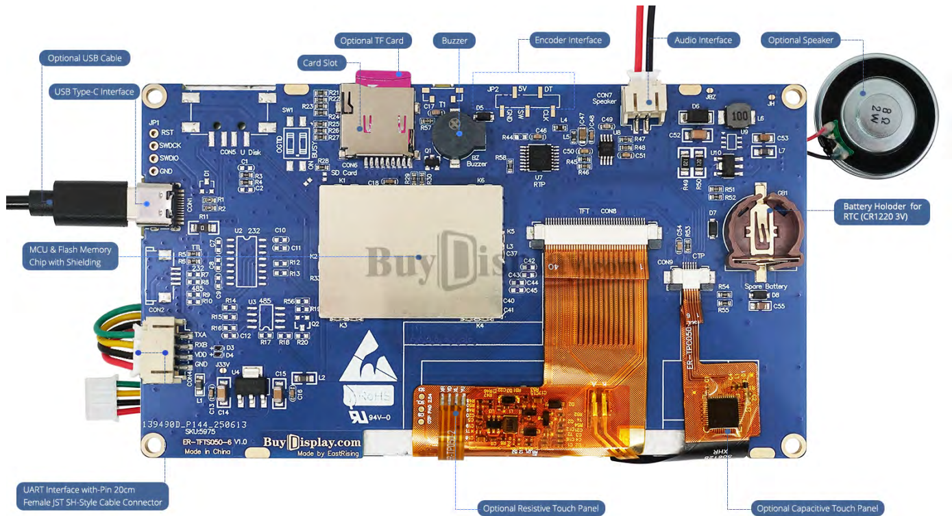
UART Board Image
