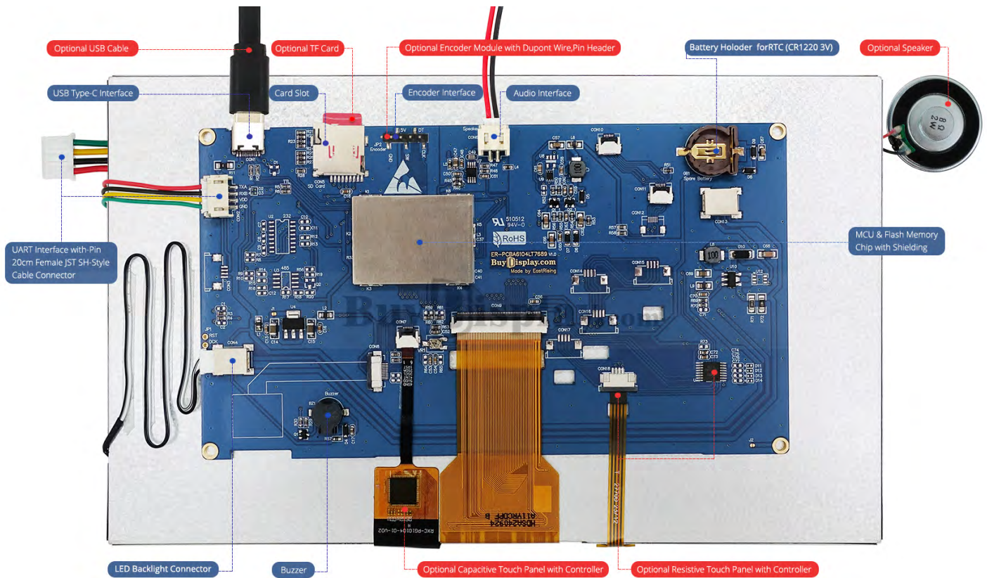
UART Board Image
