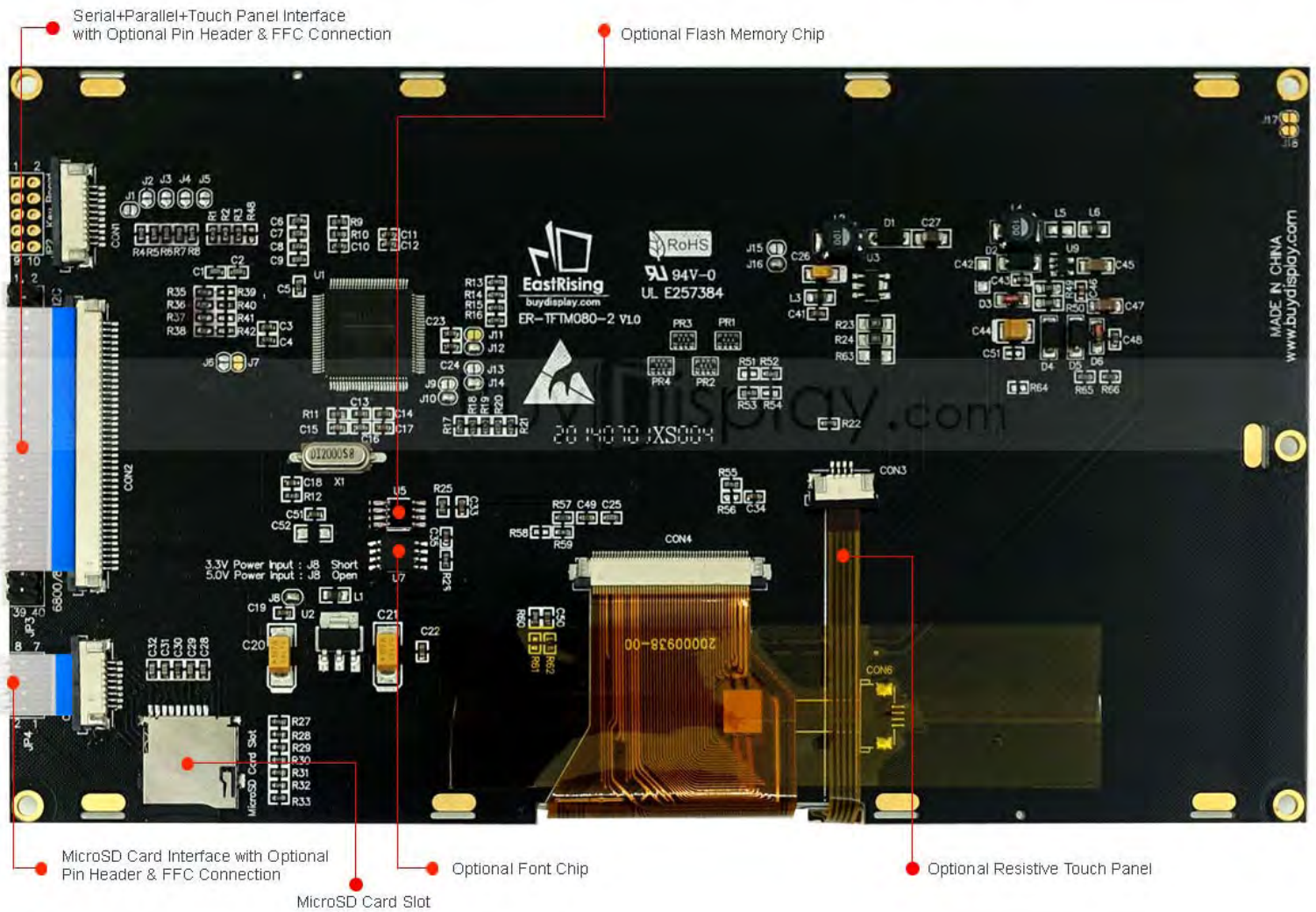
ER-TFTM080-2 Controller Board with Optional Resistive Touch Panel
