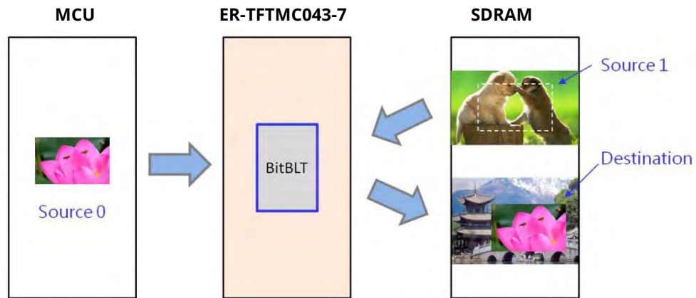
Figure 7-4: Example of MCU Write with ROP The suggested programming steps and register settings are listed below as reference.
