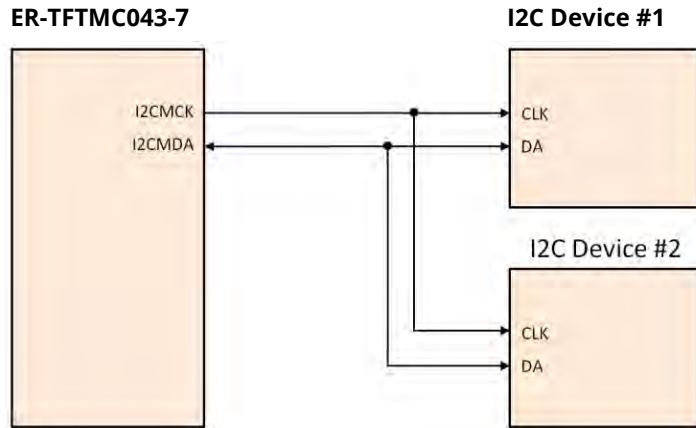
Figure 10-1: Application Circuit of ER-TFTMC043-7 I2C Master
