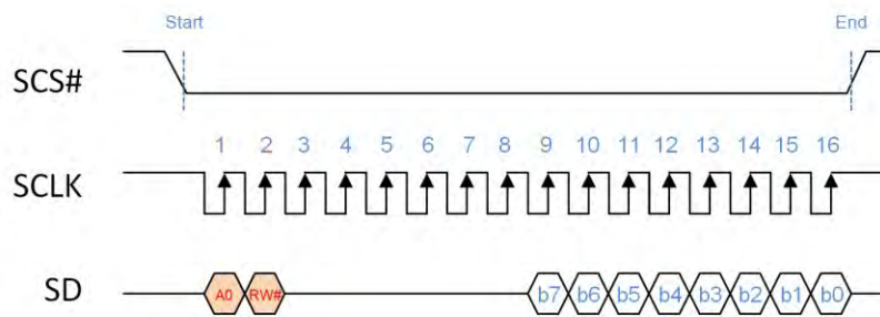
Figure 2-6: 3-Wire SPI Interface Timing
