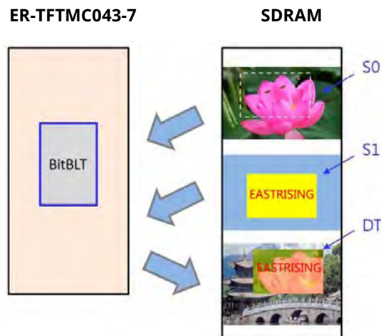
Figure 7-28: Example of Memory Copy with Opacity - Picture Mode
