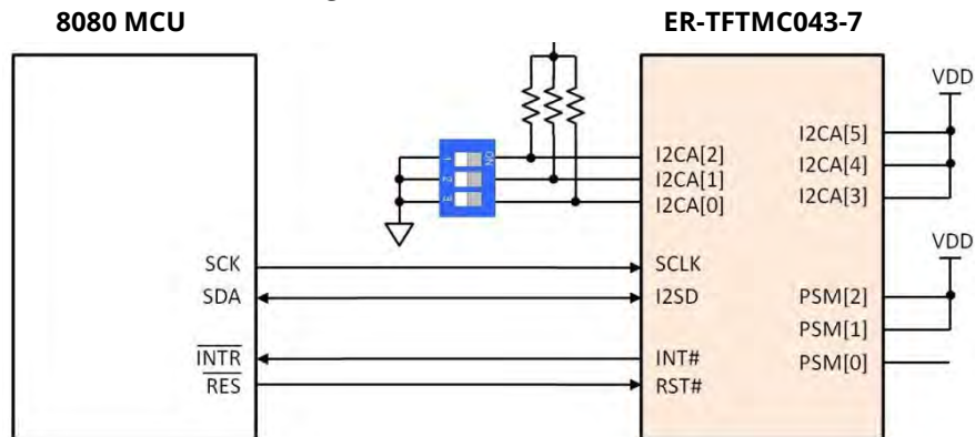
Figure 2-10: I2C Interface
