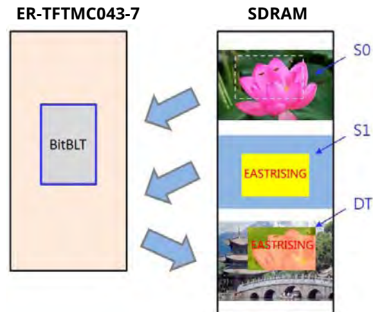
Figure 7-26: Example of Pixel Mode - 16bpp
