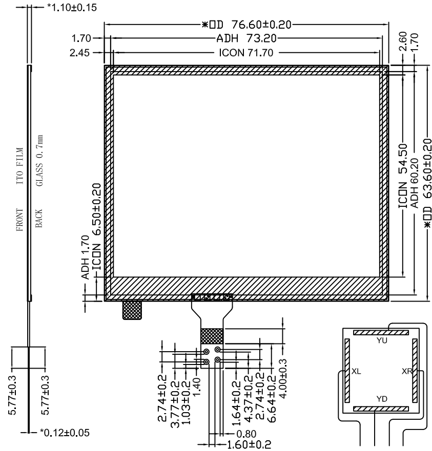
Logic Drawing
